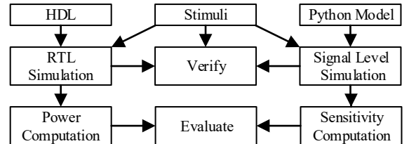
Fig. 9. The design and evaluation flow for the demodulators.
