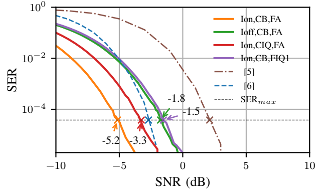
Fig. 11. Sensitivity calculation for several example configurations and the works from [6] and [5] at 40% of the maximum signal magnitude.
