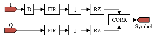
Fig. 2. Architecture of a typical 802.15.4 conformant demodulator.
