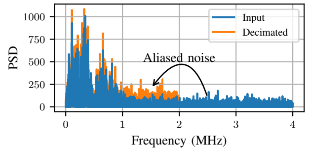
Fig. 7. The BFA impact on the signal Power Spectral Density (PSD): with bypassed filter, the noise is aliased into the baseband spectrum.
