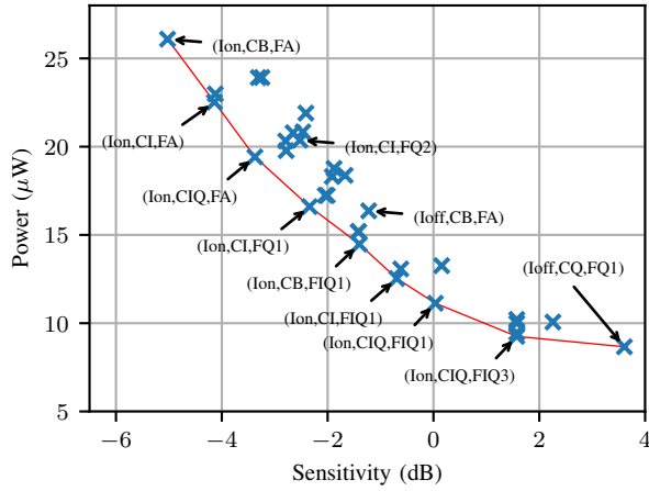
Fig. 13. Sensitivity-power trade-off with the adequate demodulator.
